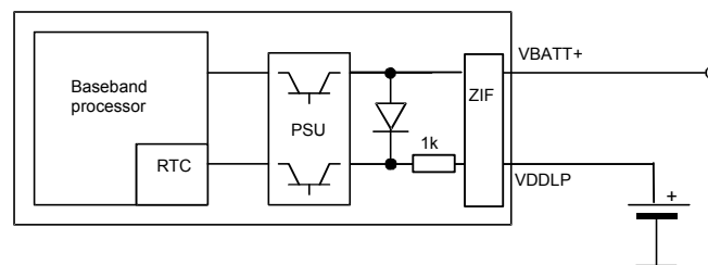
Figure 13: RTC supply from rechargeable battery (accumulator)
